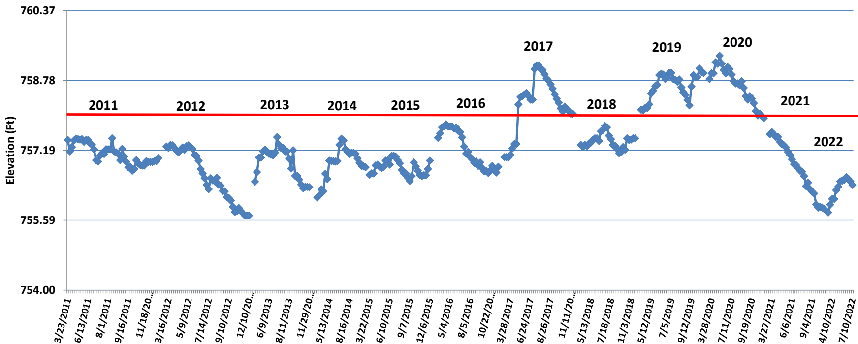
Lily Lake Water Level - 2011-22 (red line=outlet pipe at 757.9)
